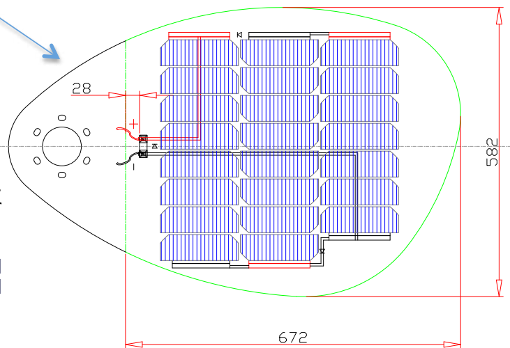
Monocrystalline semi-flexible film mounted on the petal
